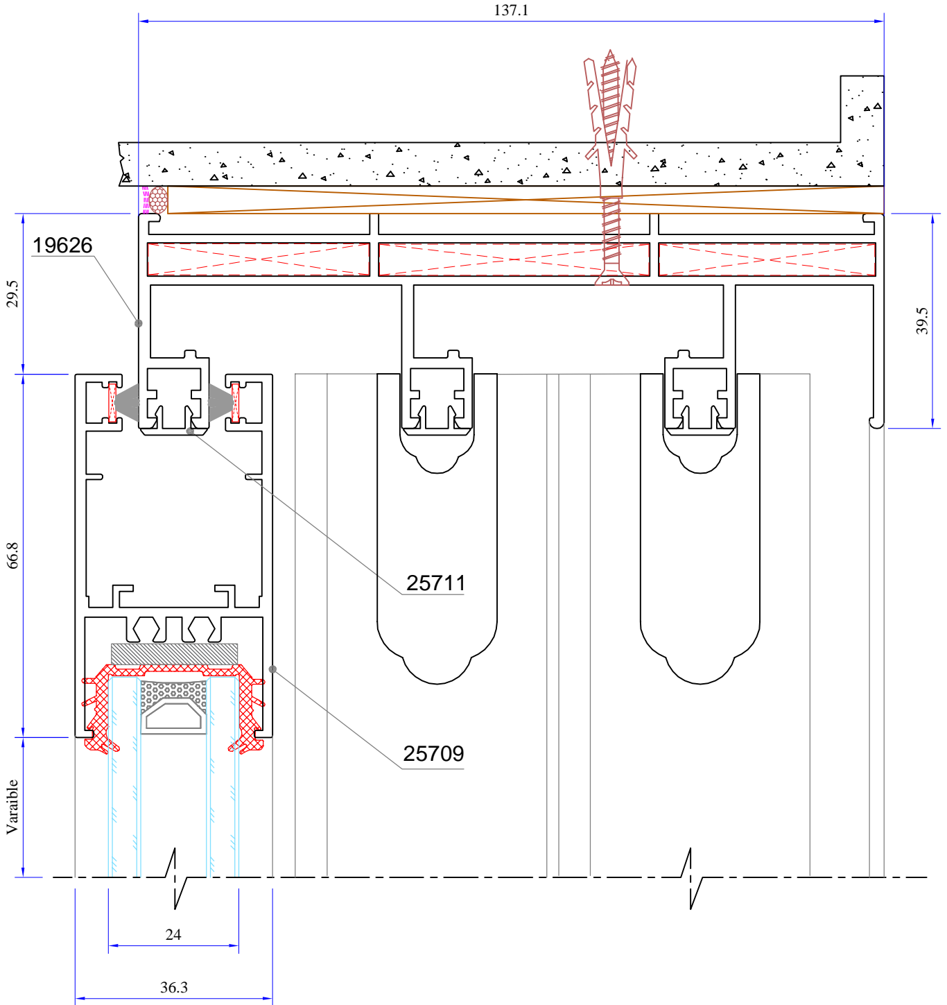
DETAIL - I
