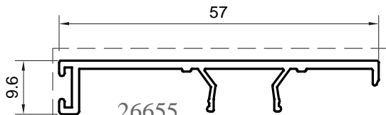
26655 (0.323 kg/m) Clip Frame for Montana 129
