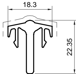
26187 (0.326 kg/m) Clip for Bottom Frame Montana 120 & 129
